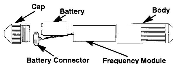
Battery Replacement
